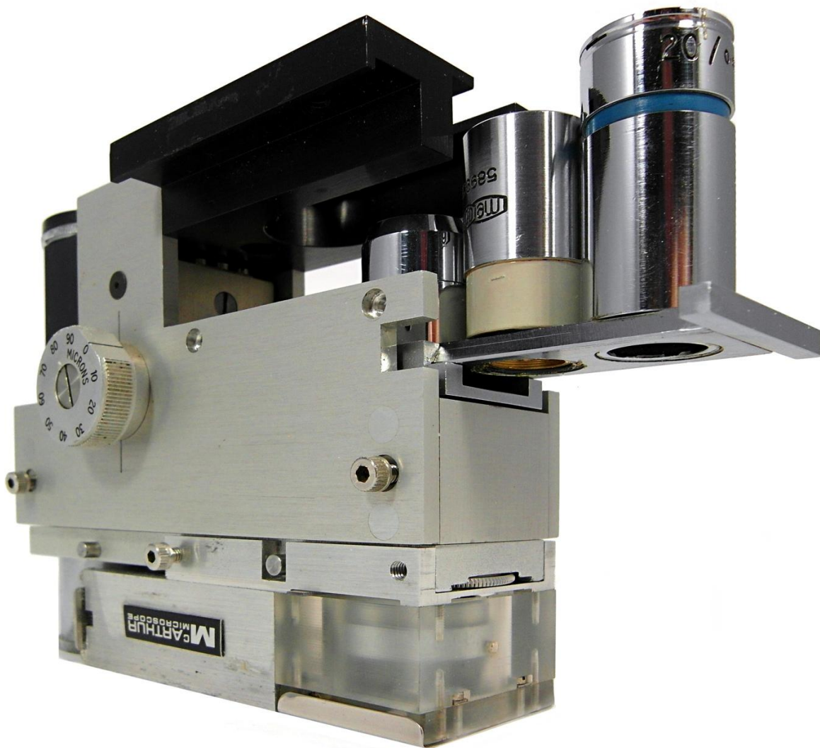
Figure 4. McArthur microscope with objectives, by Vickers, Meopta and Cooke. Its stage is located on the top, and it has sub-lens illumination.
